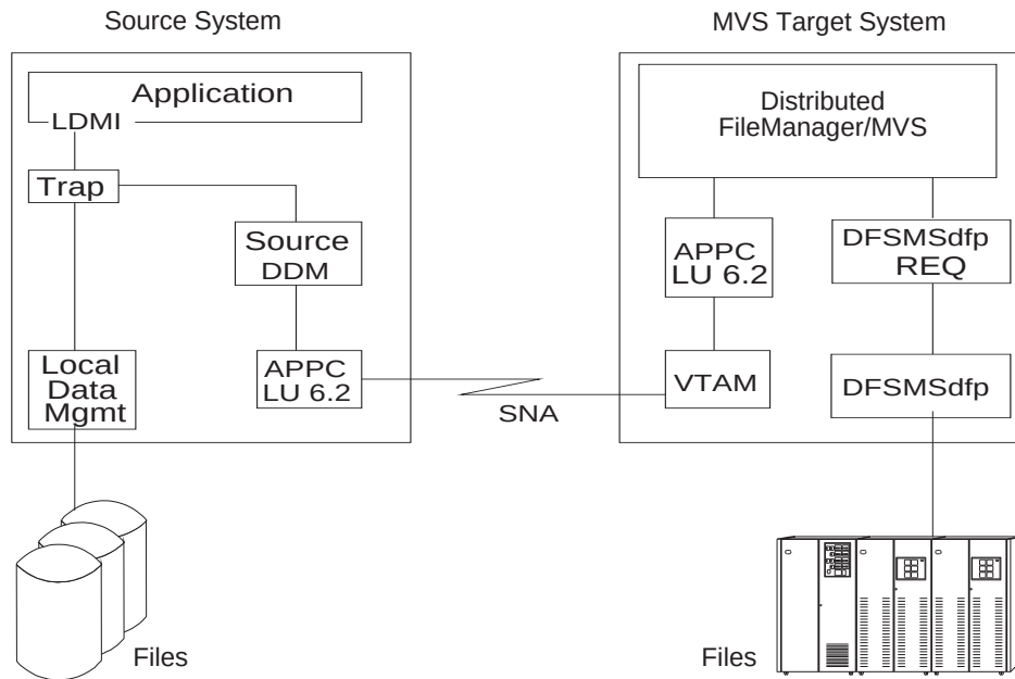
Figure 5. DDM Source System/MVS Target Communication Flow
